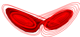
Figure 13-3 Three-dimensional model of a strange attractor.
